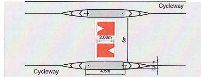
Proposed Speed Cushion & Islands
