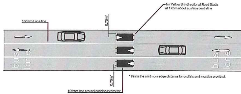
Proposed 3-Lane Traffic Cushion Layout
