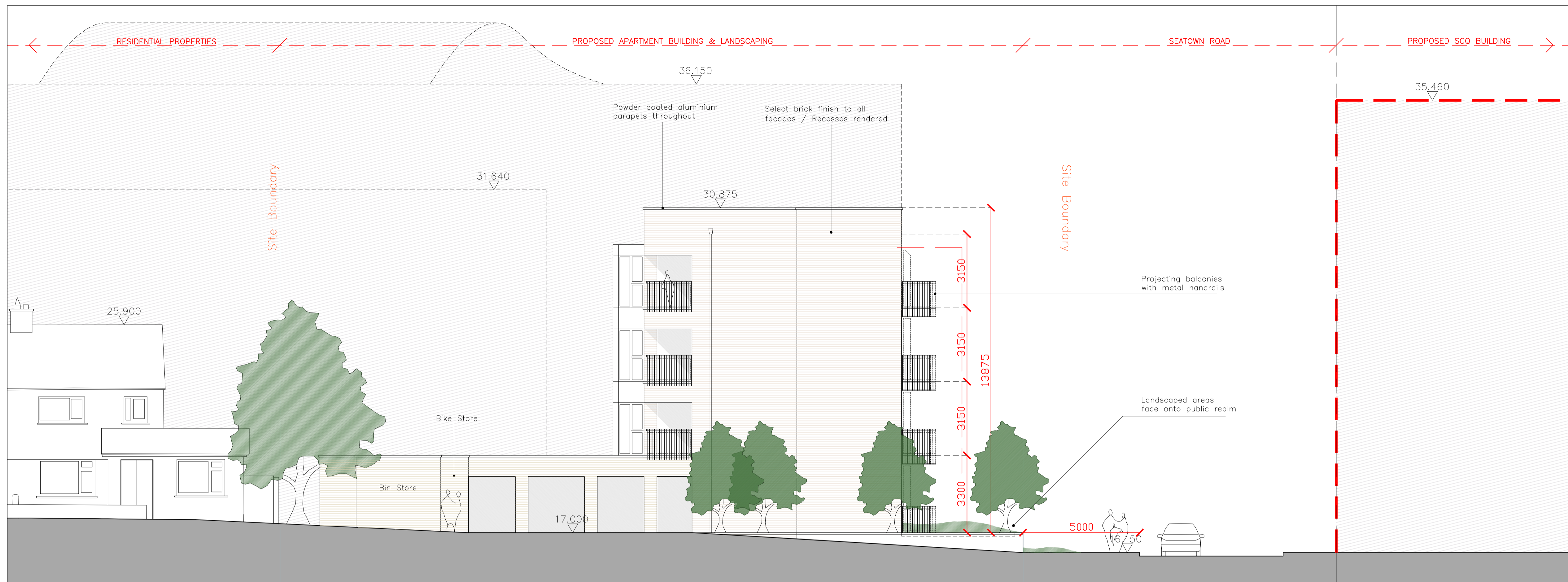
SITE NO 2 - PROPOSED SECTIONAL ELEVATION S2C (NORTH EAST) / SCALE 1:100
