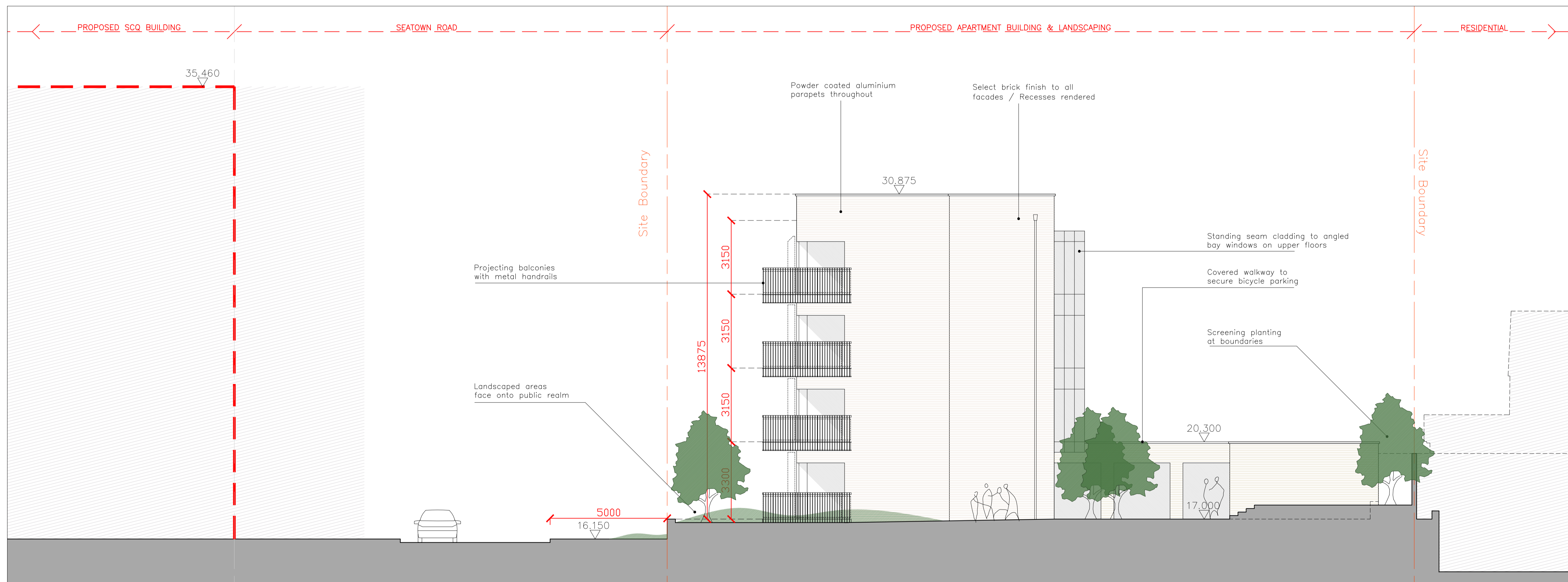
SITE NO 2 - PROPOSED SECTIONAL ELEVATION S2D (SOUTH WEST) / SCALE 1:100
