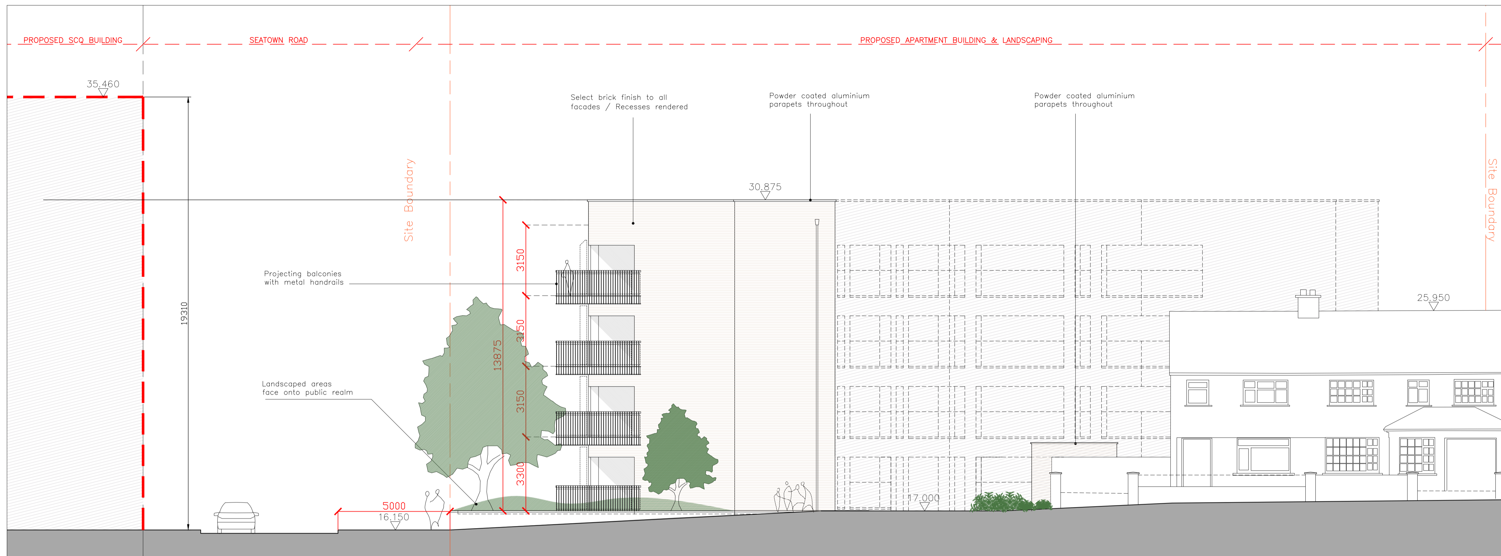
SITE NO 1 - PROPOSED SECTIONAL ELEVATION S1C (SOUTH WEST) / SCALE 1:100
