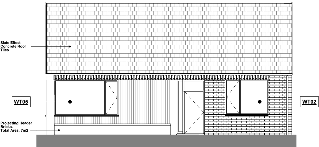
4 West Elevation_House Type B2 1 : 50
