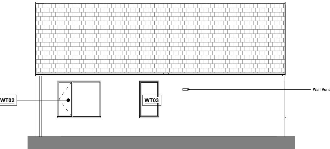
3 East Elevation_House Type B2 1 : 50
