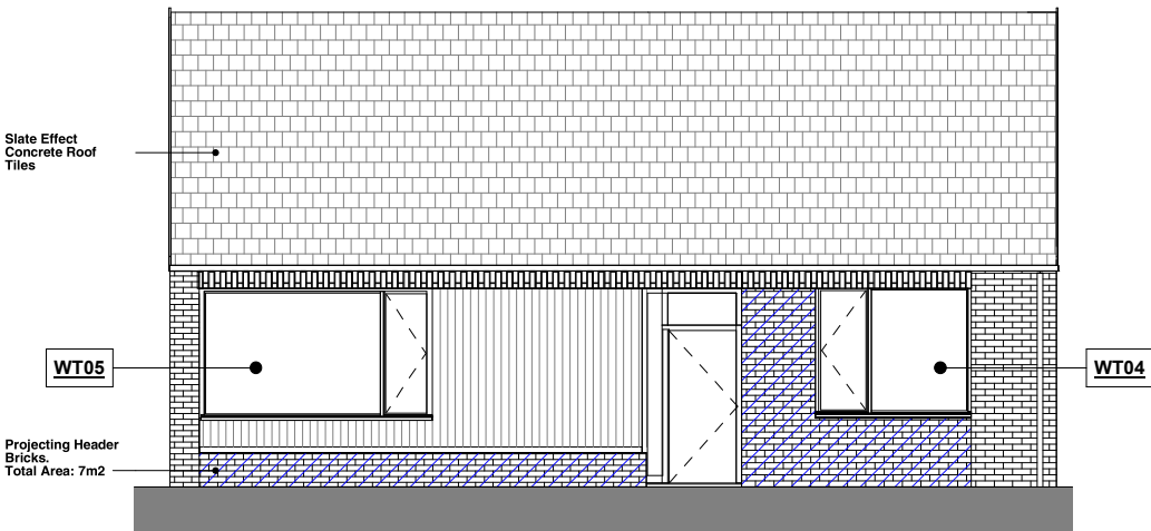
4 West Elevation_House Type B1 1 : 50
