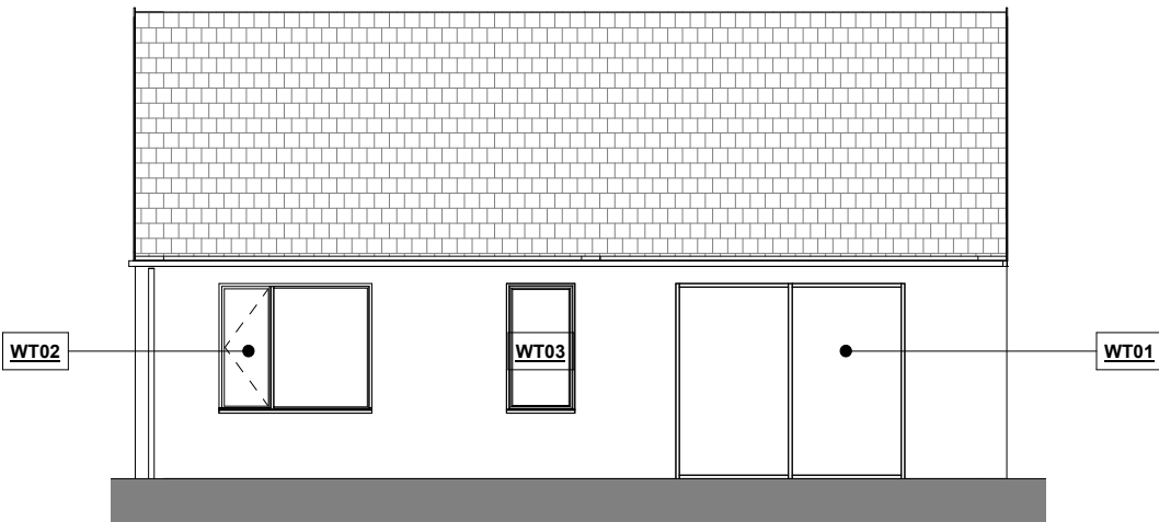
3 East Elevation_House Type B1 1 : 50
