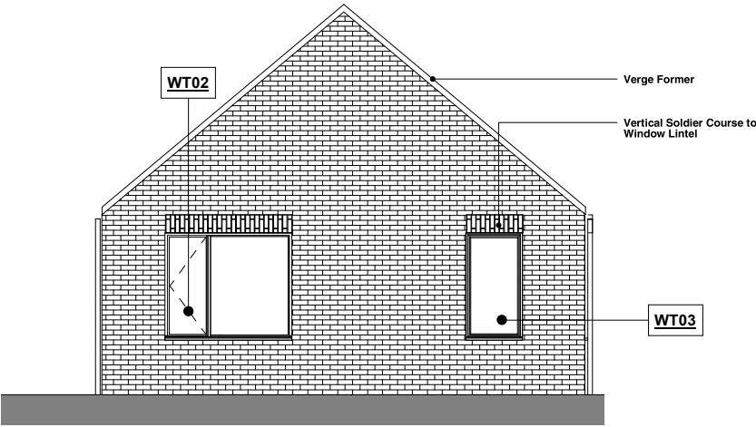
2 South Elevation_House Type A1 1 : 50
