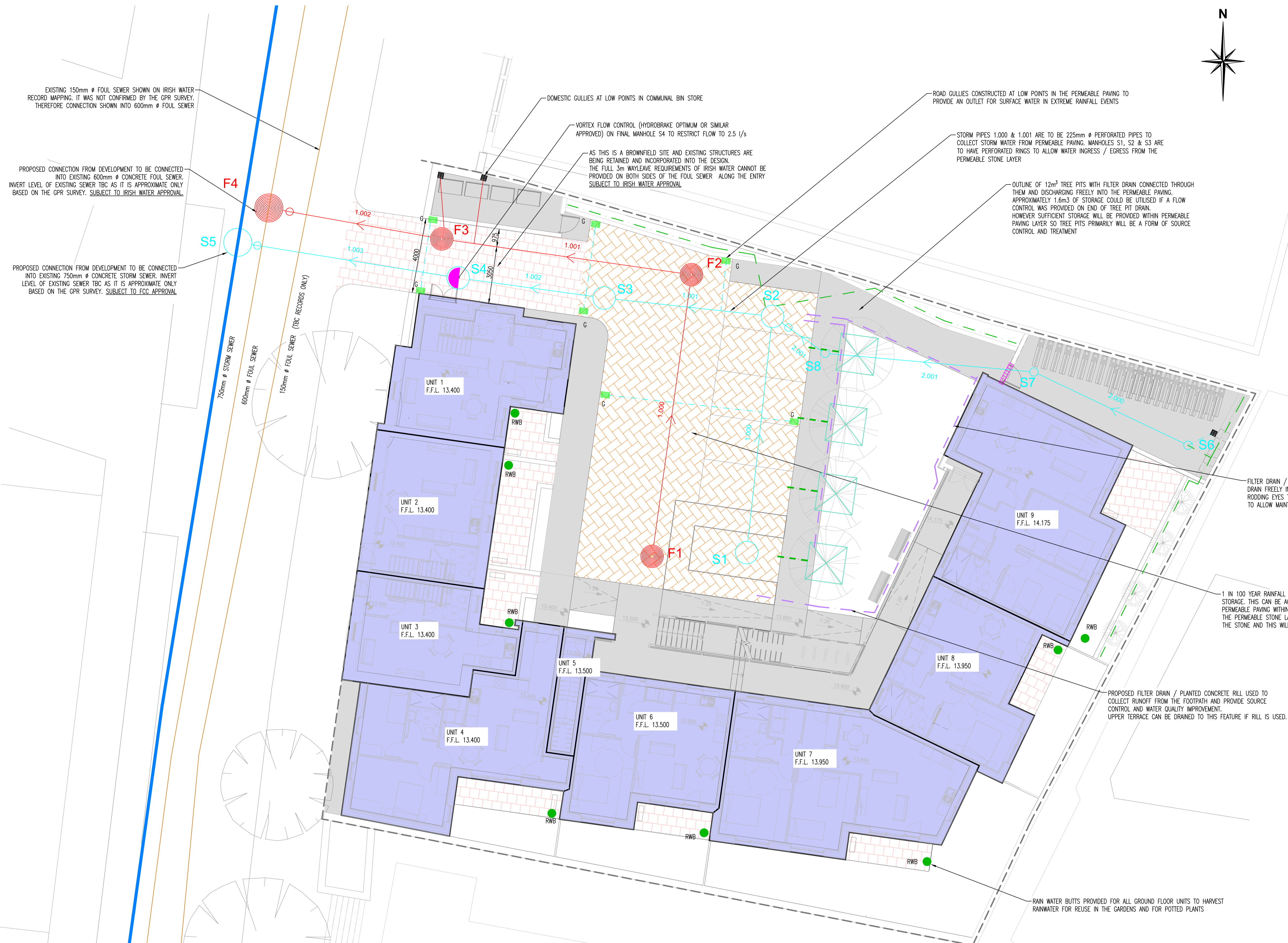
PROPOSED DRAINAGE LAYOUT SCALE 1:100
