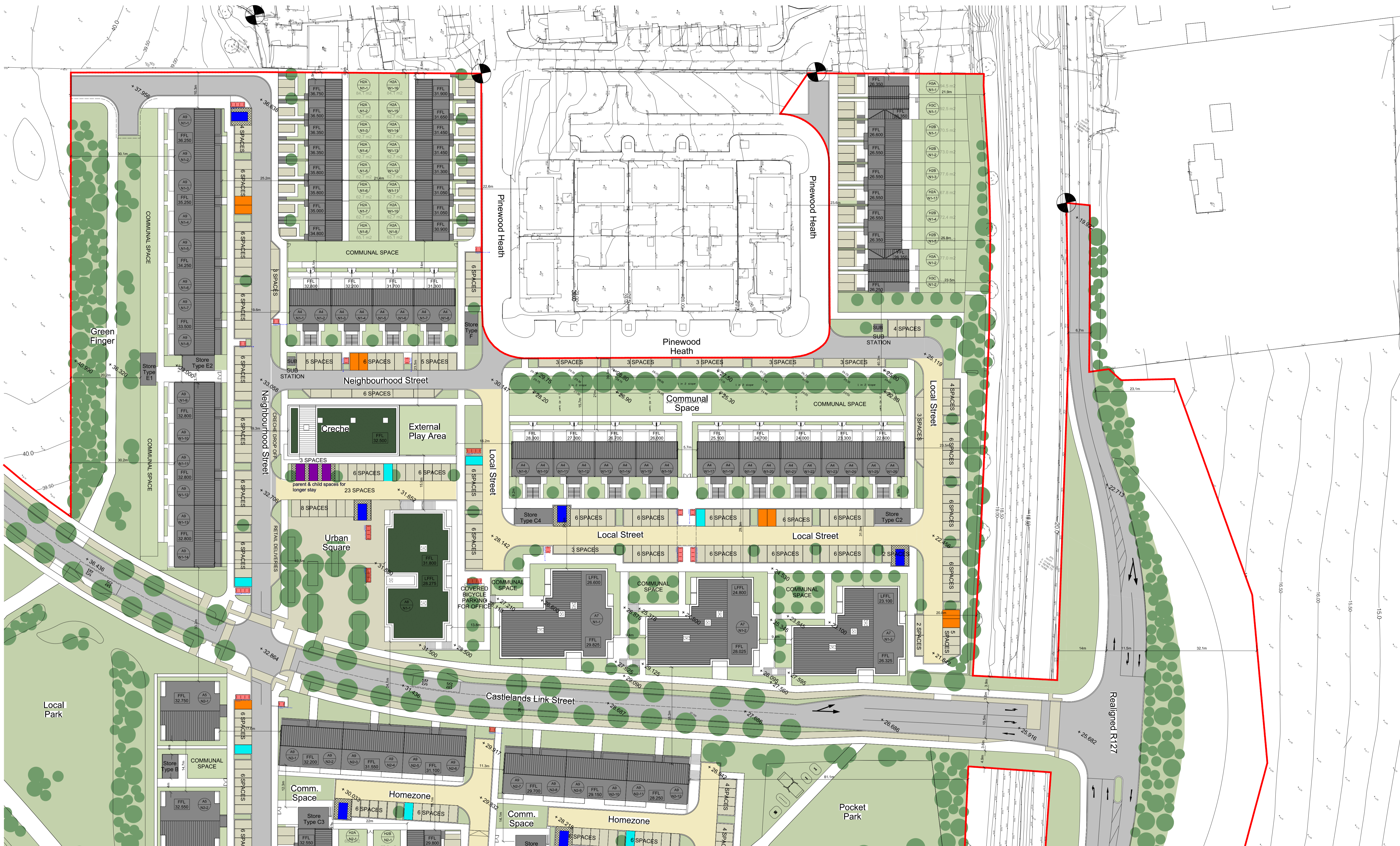
Proposed Site Layout Plan_Neighbourhood 1
