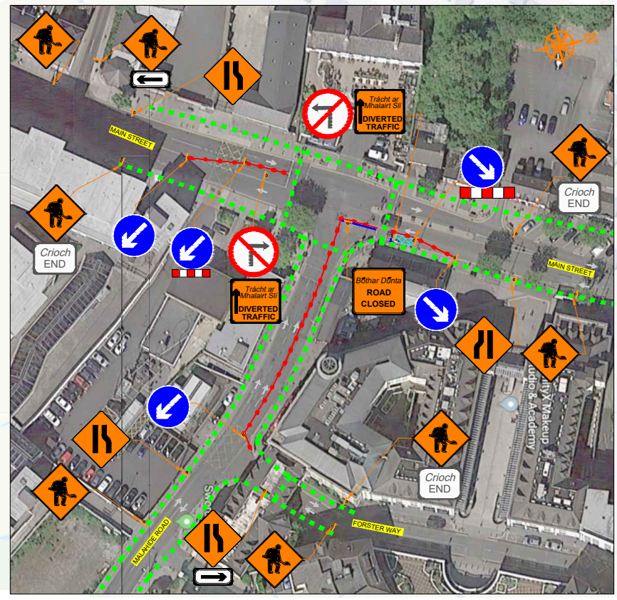
DETAIL A MAIN STREET JUNCTION CLOSURE
