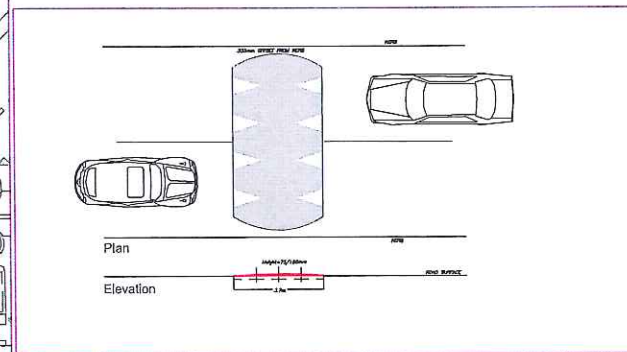
Traffic Calming Ramp Not to Scale
