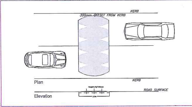
Traffic Calming Ramp Not to Scale
