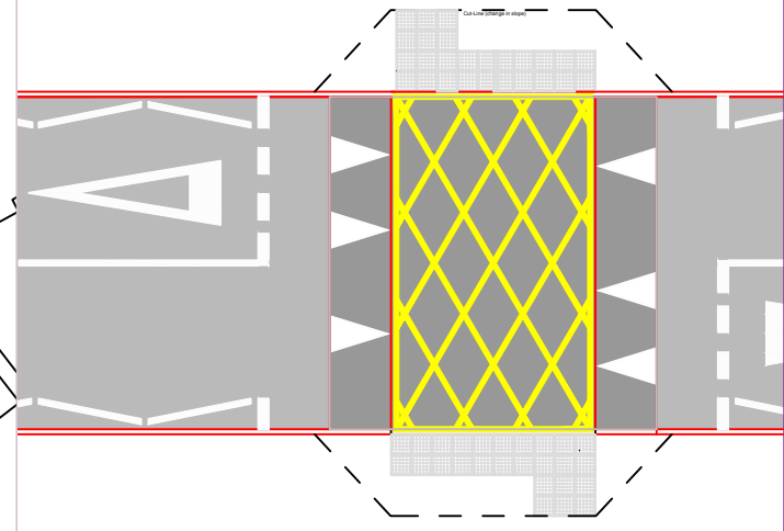
Traffic Calming Ramp Not to Scale
