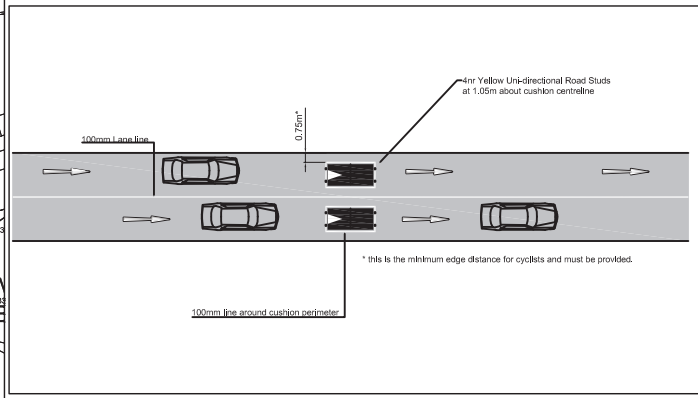
Traffic Calming Ramp Not to Scale
