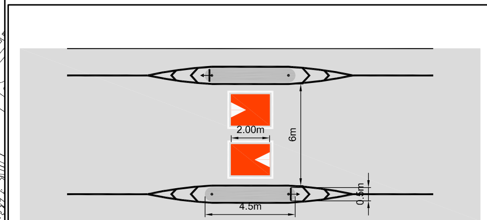
Proposed Speed Cushion & Islands
