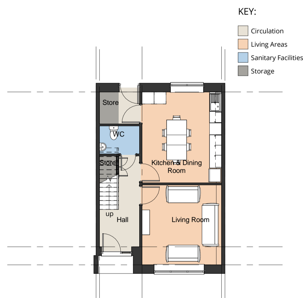
6 HT - C Ground Floor Plan 1 : 100
