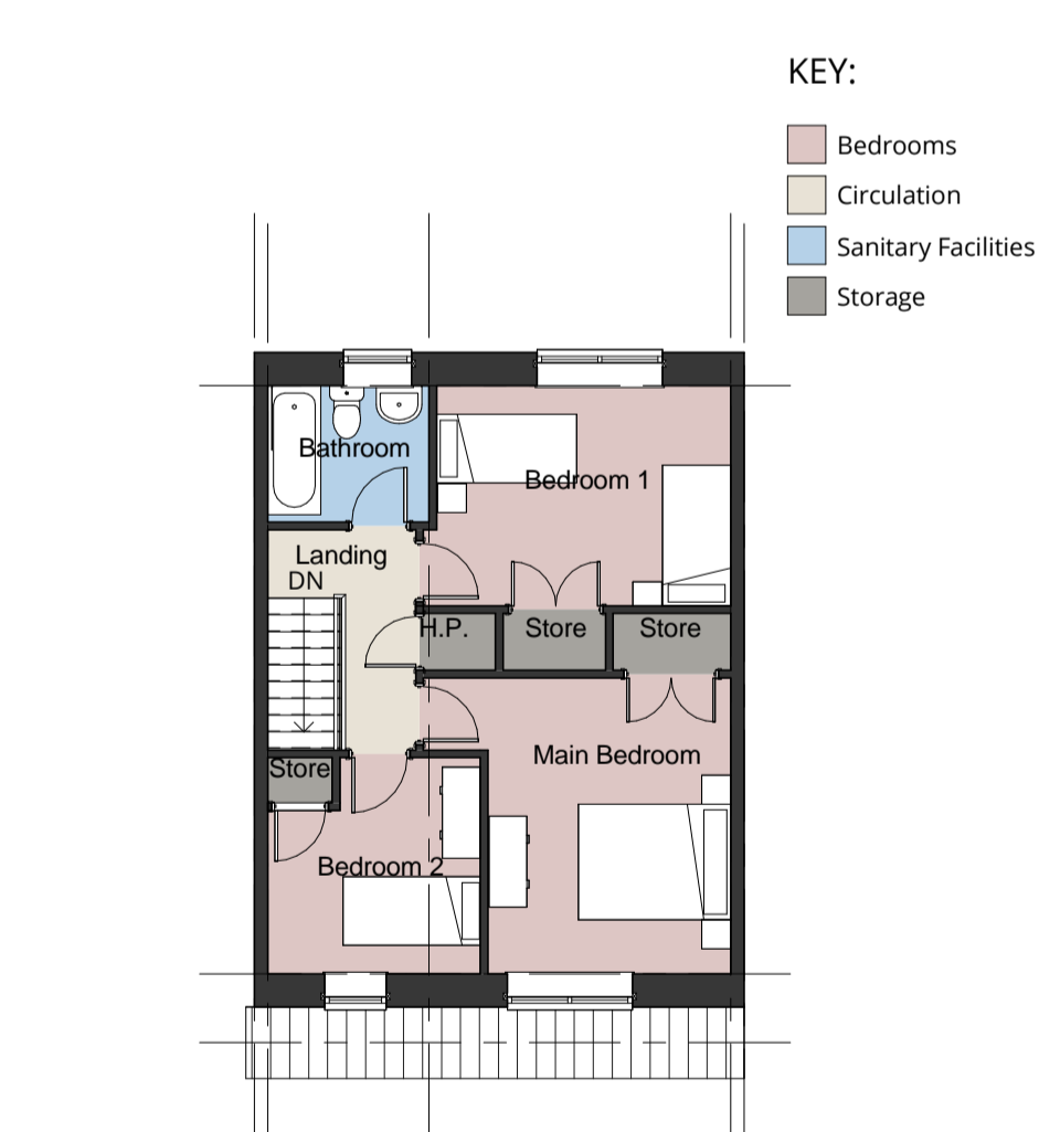
7 HT - C First Floor Plan 1 : 100
