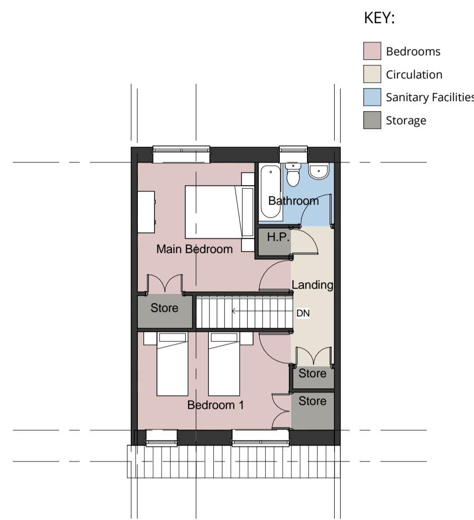
2 HT - B First Floor Plan 1 : 100
