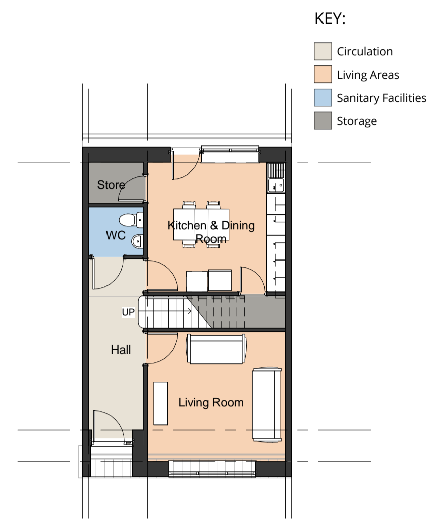
1 HT - B Ground Floor Plan 1 : 100
