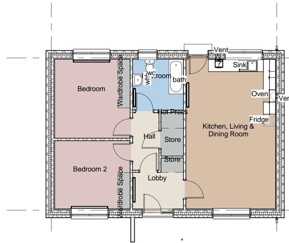
5 HT - A Ground Floor Plan 1 : 100
