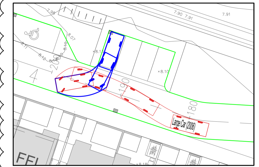
INSERT B LARGE CAR SWEEP PATH REVERSE ENTRY TO PUBLIC PARKING BAY SCALE 1:250
