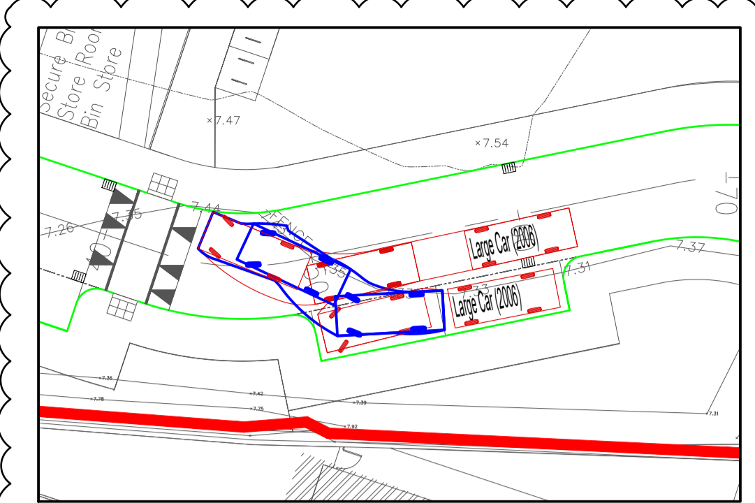
INSERT A LARGE CAR SWEEP PATH REVERSE ENTRY TO PUBLIC PARKING BAY SCALE 1:250
