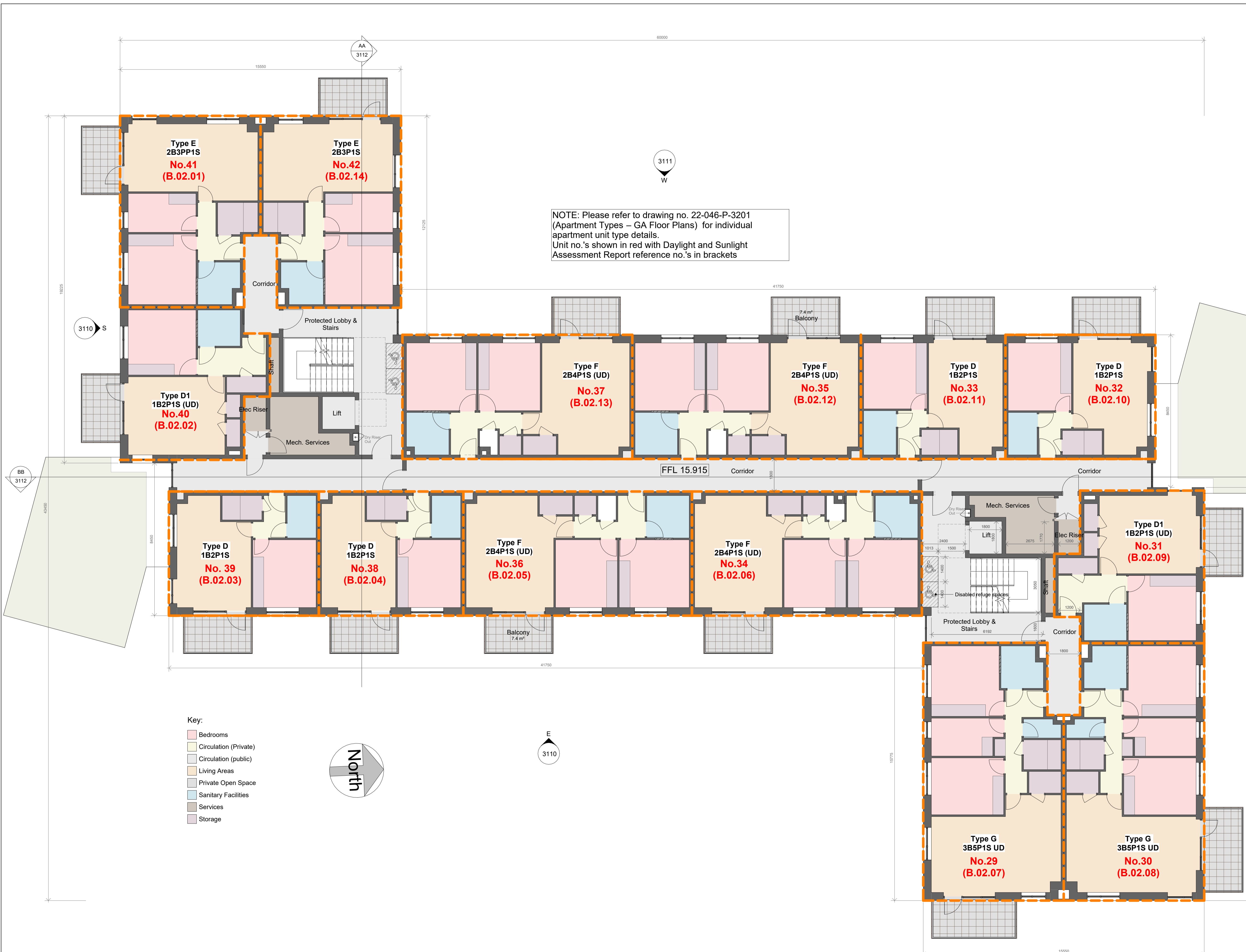
APARTMENT BLOCK - SECOND FLOOR PLAN 1 : 100 @ A1
