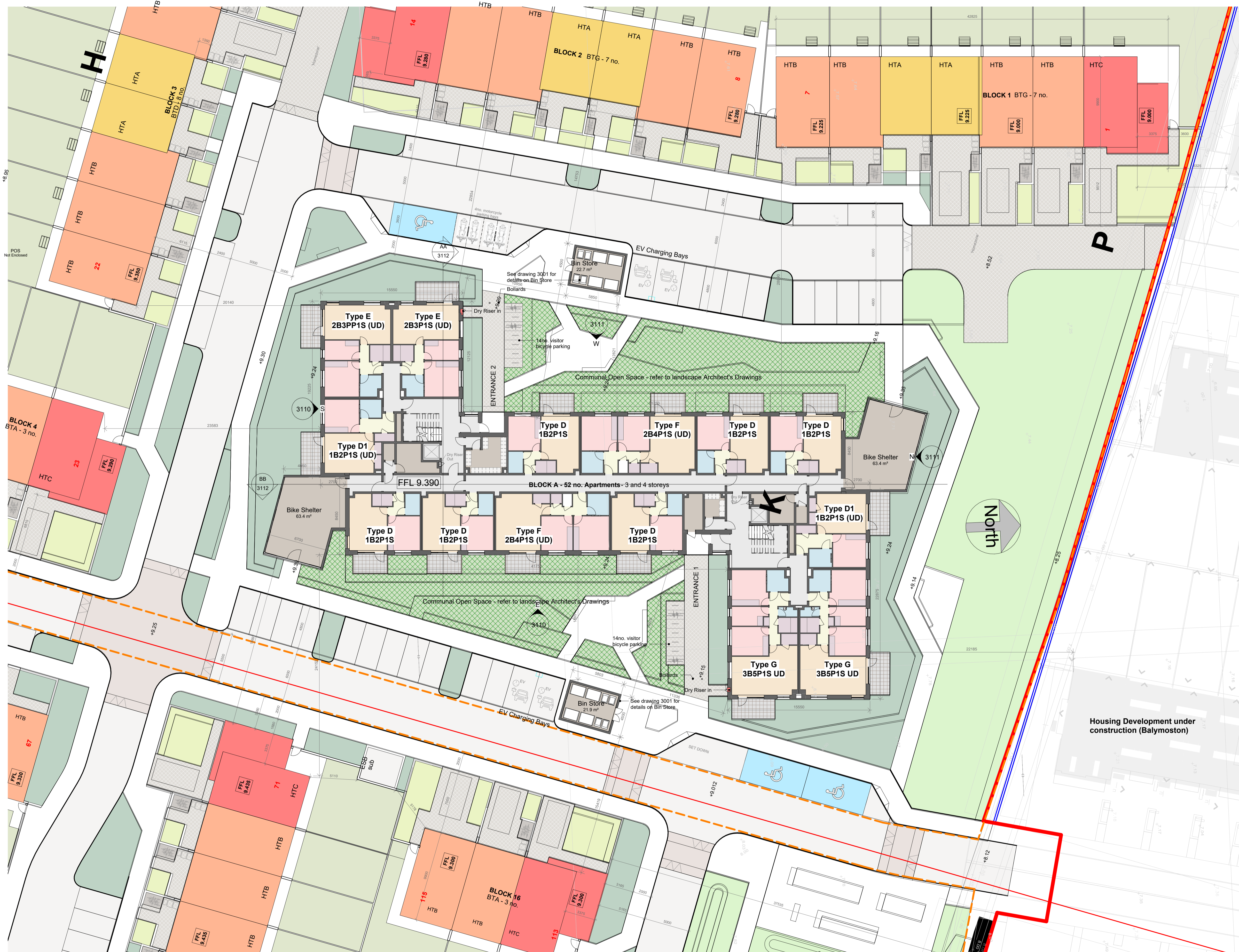
APARTMENT BLOCK - SITE PLAN 1 : 200 @ A1
