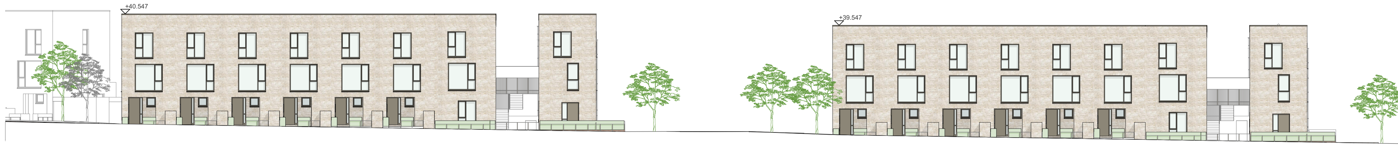
E-01 ELEVATION SOUTHEAST BLOCK 3A AND 3B - TO LINK STREET P3301 1:200
