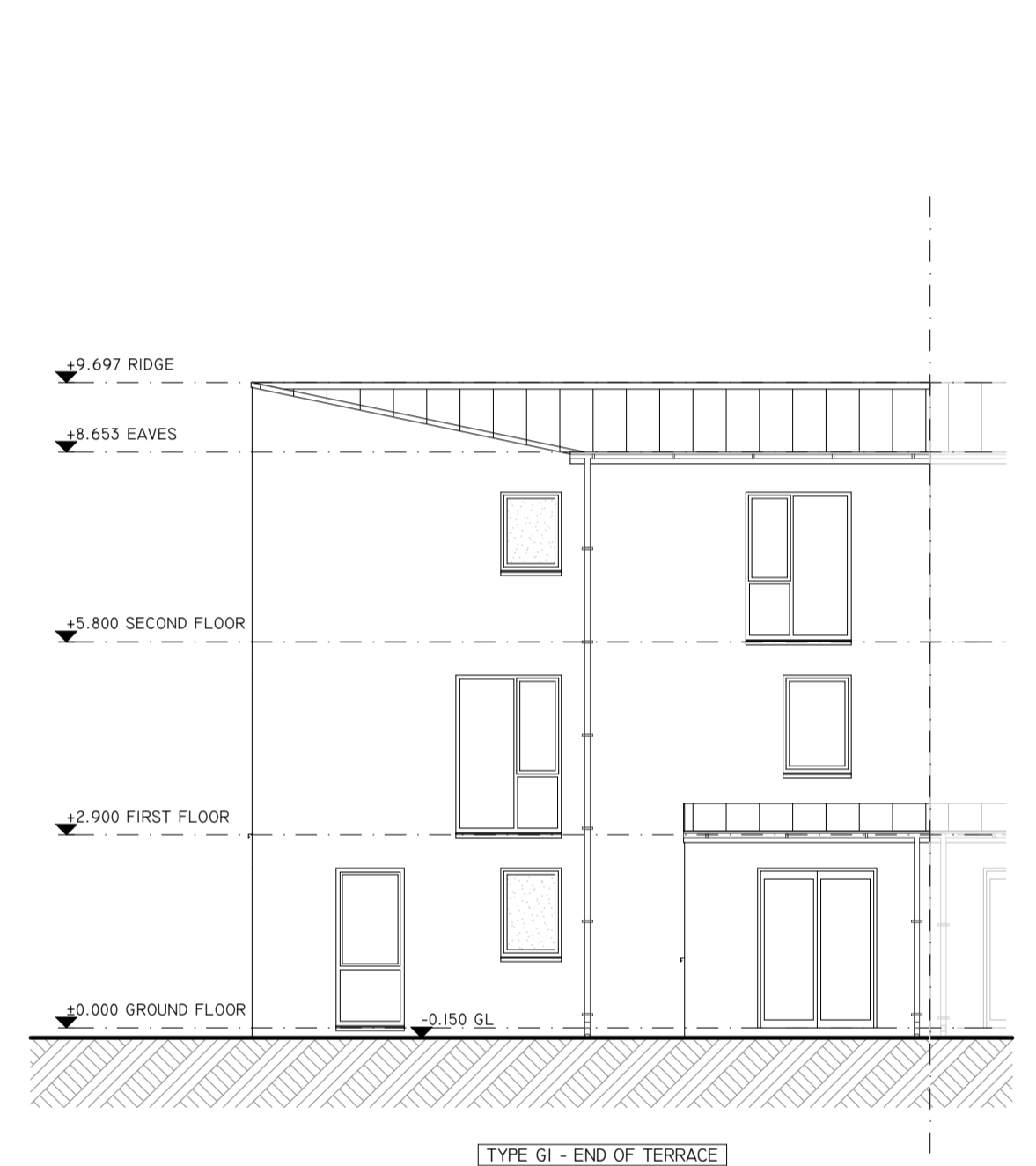
13 REAR ELEVATION PI013 1:100 TYPE G1 - END OF TERRACE
