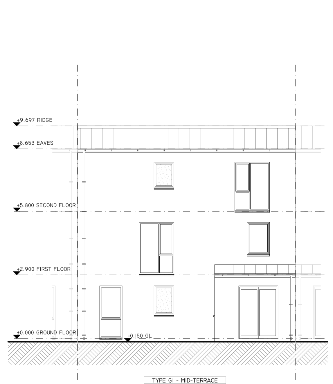
12 REAR ELEVATION PI013 1:100 TYPE G1 - MID-TERRACE
