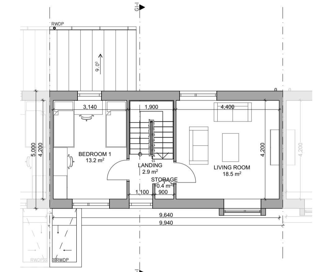
3 FIRST FLOOR PI013 1:100 TYPE G1 - MID-TERRACE
