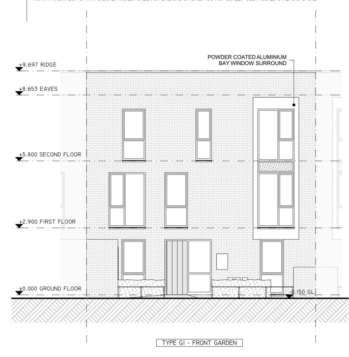
11 FRONT ELEVATION - GARDEN PI013 1:100 TYPE G1 - FRONT GARDEN
