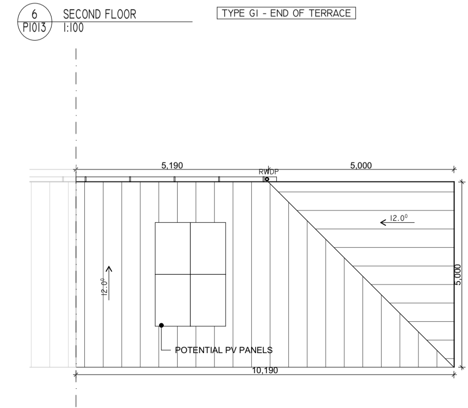
8 ROOF LEVEL PI013 1:100 TYPE G1 - END OF TERRACE
