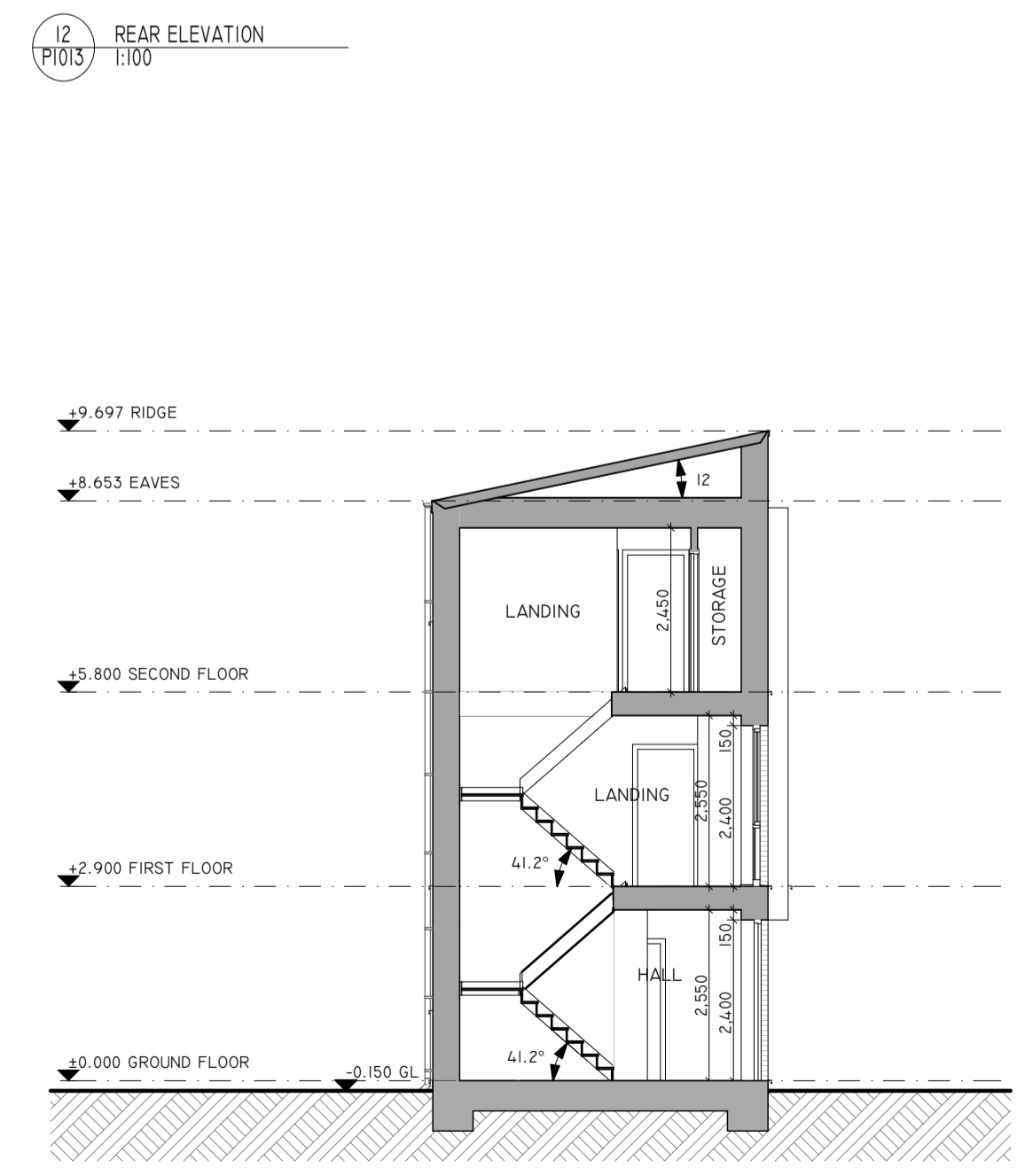
14 SECTION PI013 1:100 TYPE G1 - CROSS SECTION
