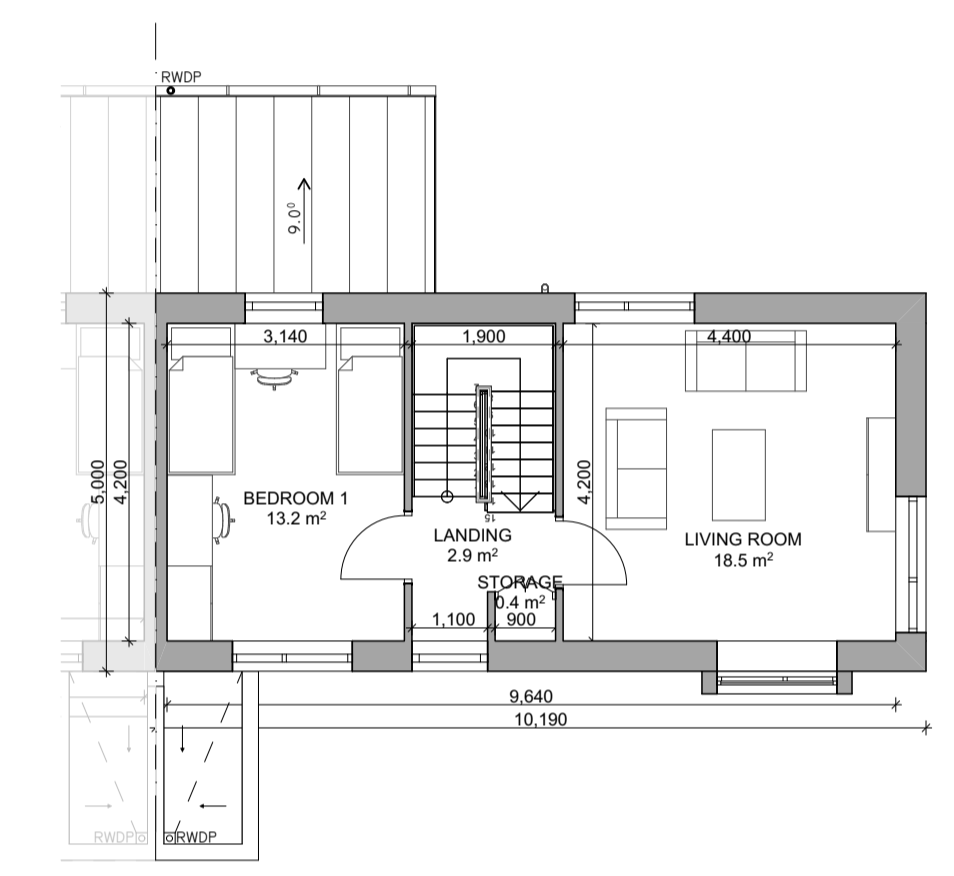
4 FIRST FLOOR PI013 1:100 TYPE G1 - END OF TERRACE
