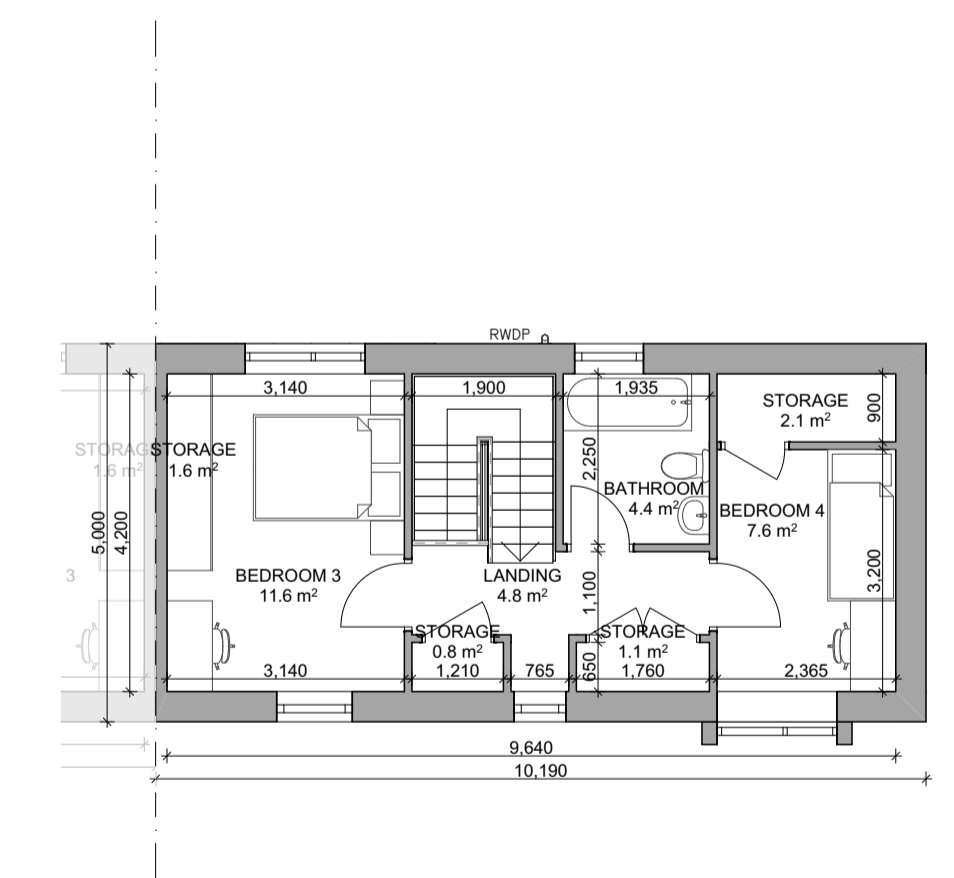
6 SECOND FLOOR PI013 1:100 TYPE G1 - END OF TERRACE
