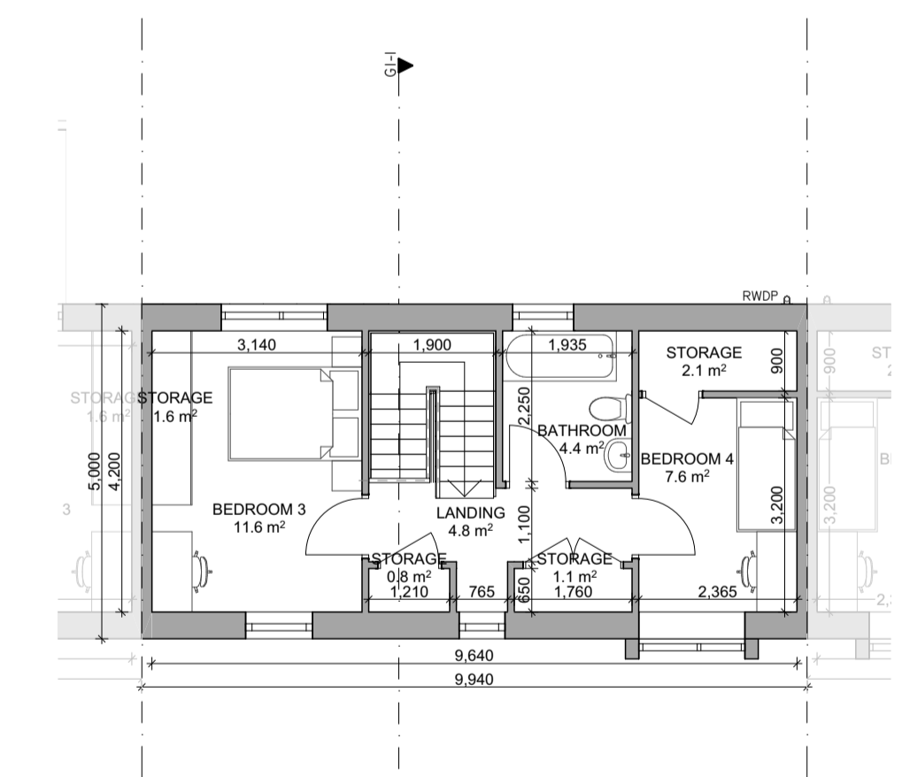
5 SECOND FLOOR PI013 1:100 TYPE G1 - MID-TERRACE
