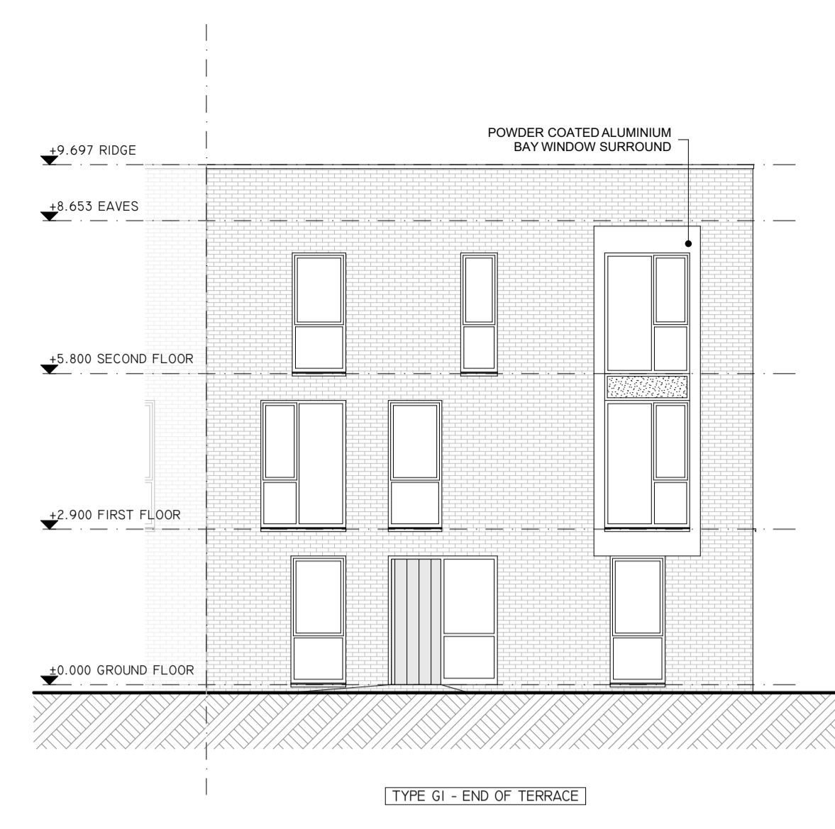
10 FRONT ELEVATION PI013 1:100 TYPE G1 - END OF TERRACE
