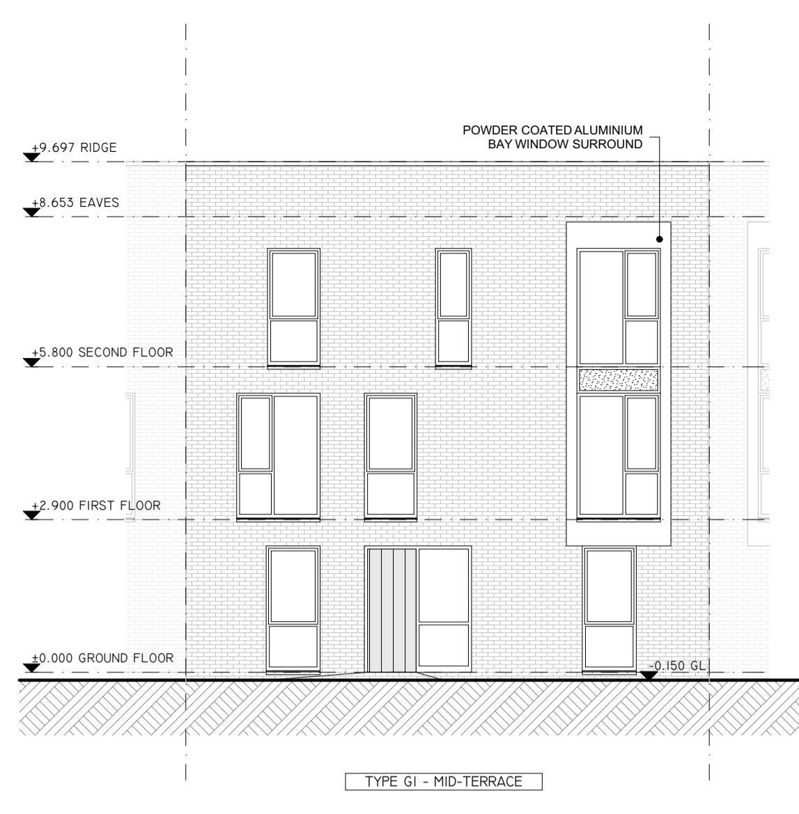
9 FRONT ELEVATION PI013 1:100 TYPE G1 - MID-TERRACE
