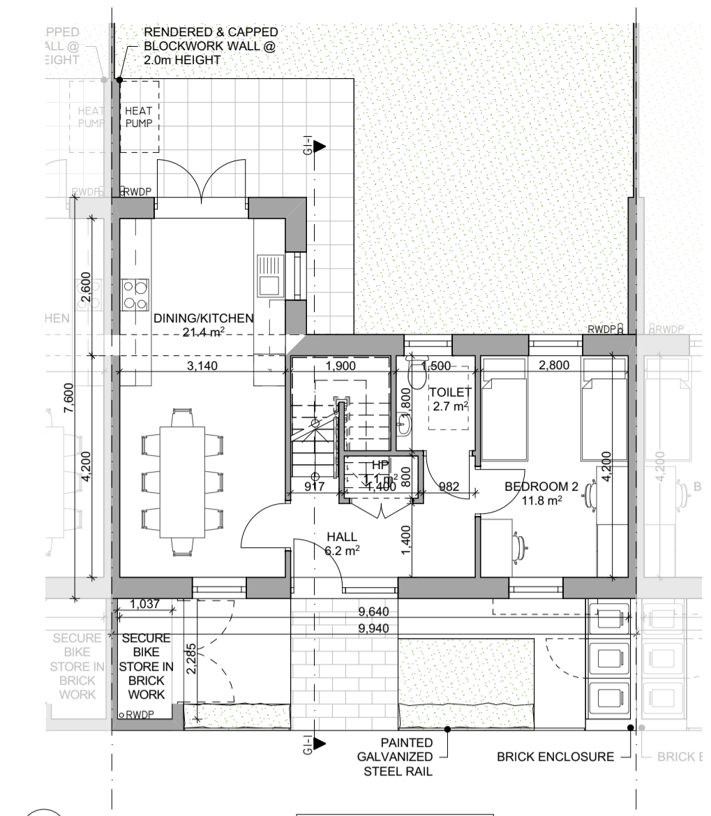
1 GROUND FLOOR PI013 1:100 TYPE G1 - MID-TERRACE
