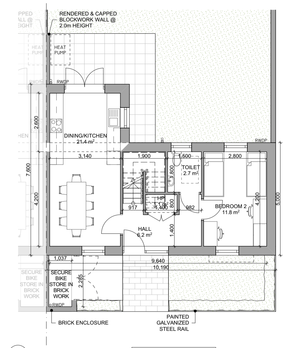
2 GROUND FLOOR PI013 1:100 TYPE G1 - END OF TERRACE
