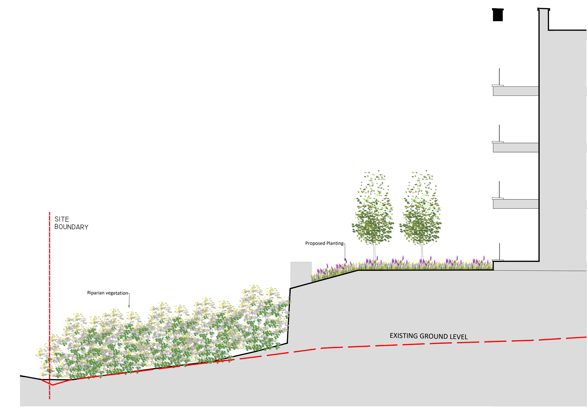
SECTION 5 Scale 1:200
