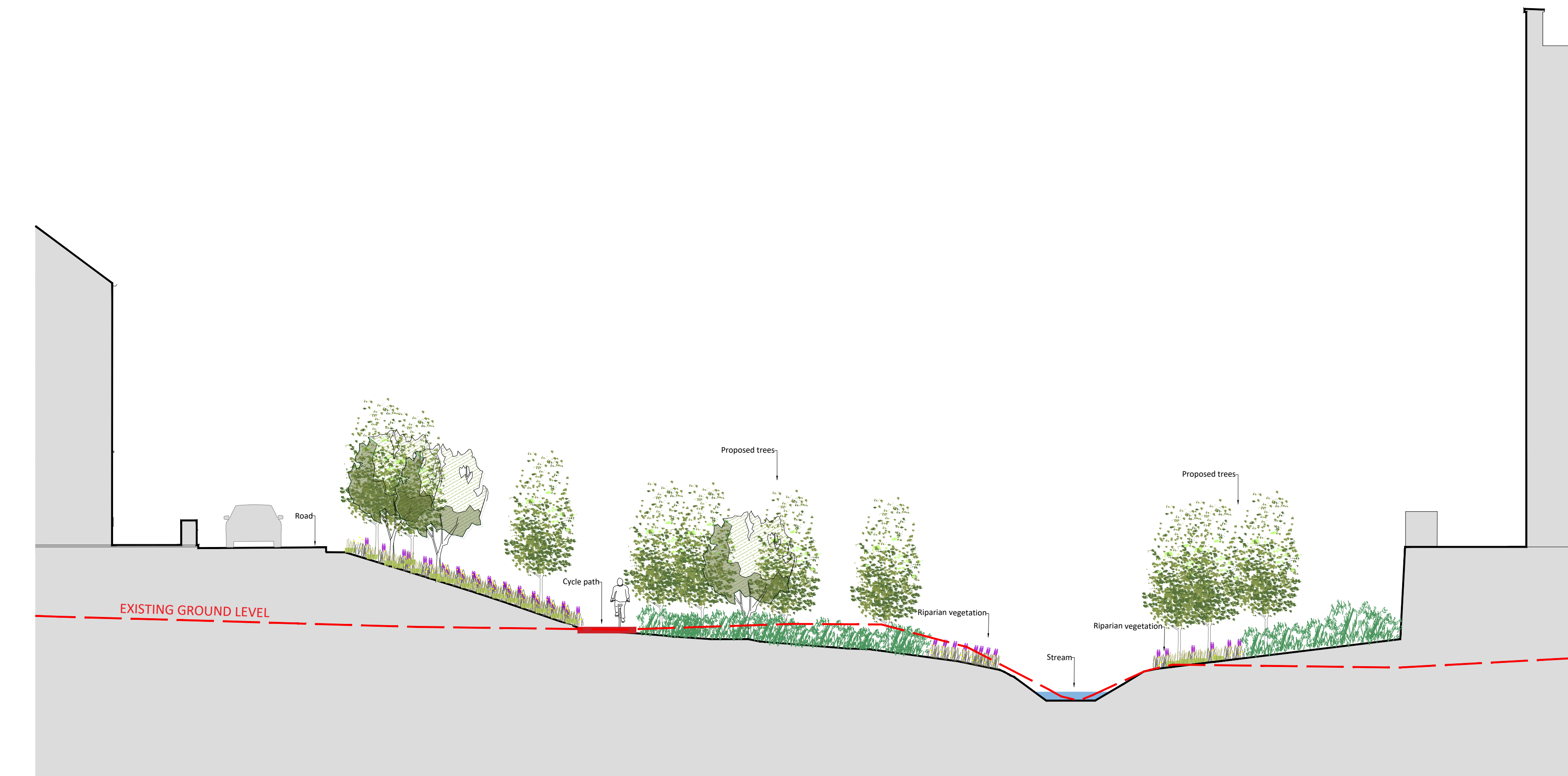
SECTION 4 Scale 1:200
