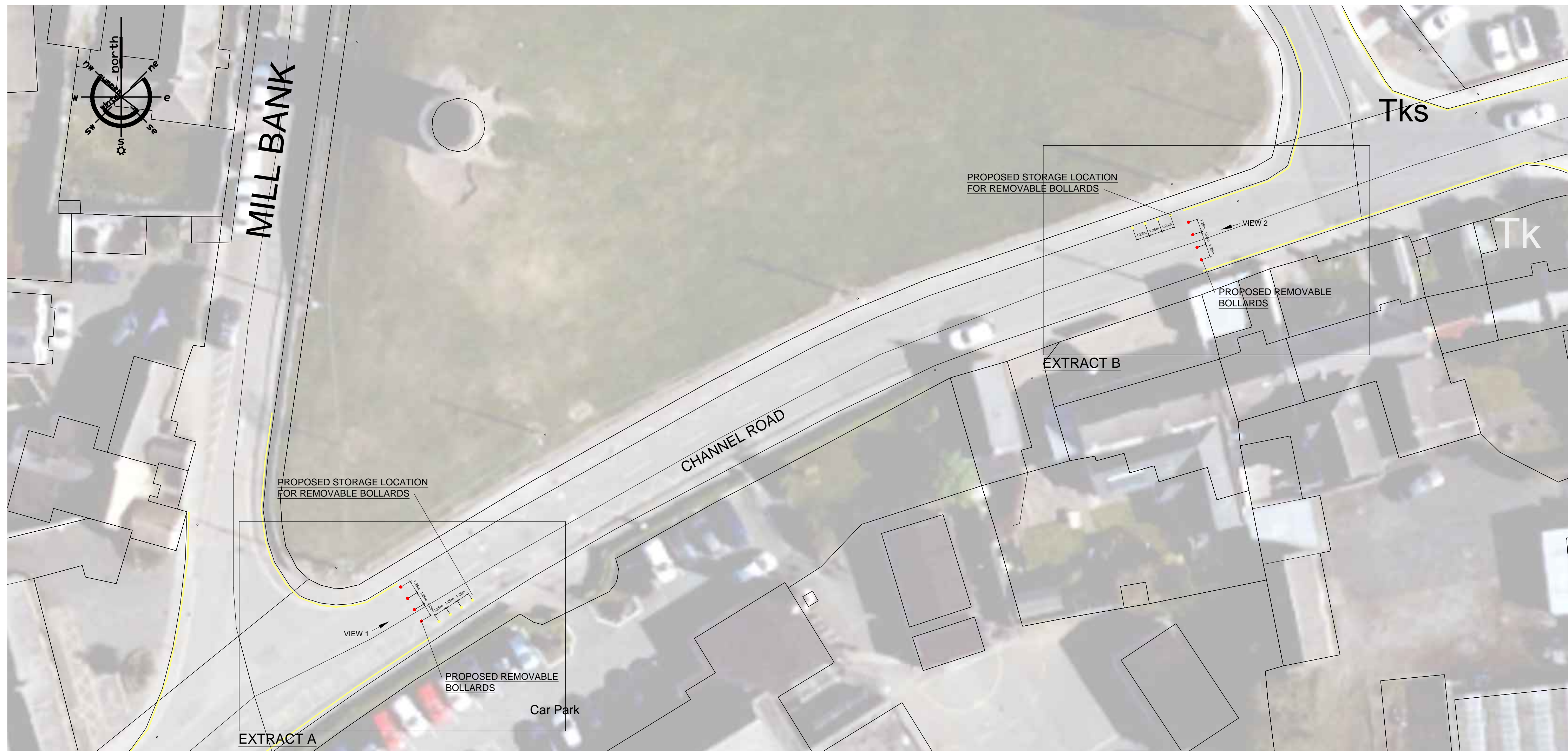
TEMPORARY ROAD CLOSURE SET - OUT Scale 1:250
