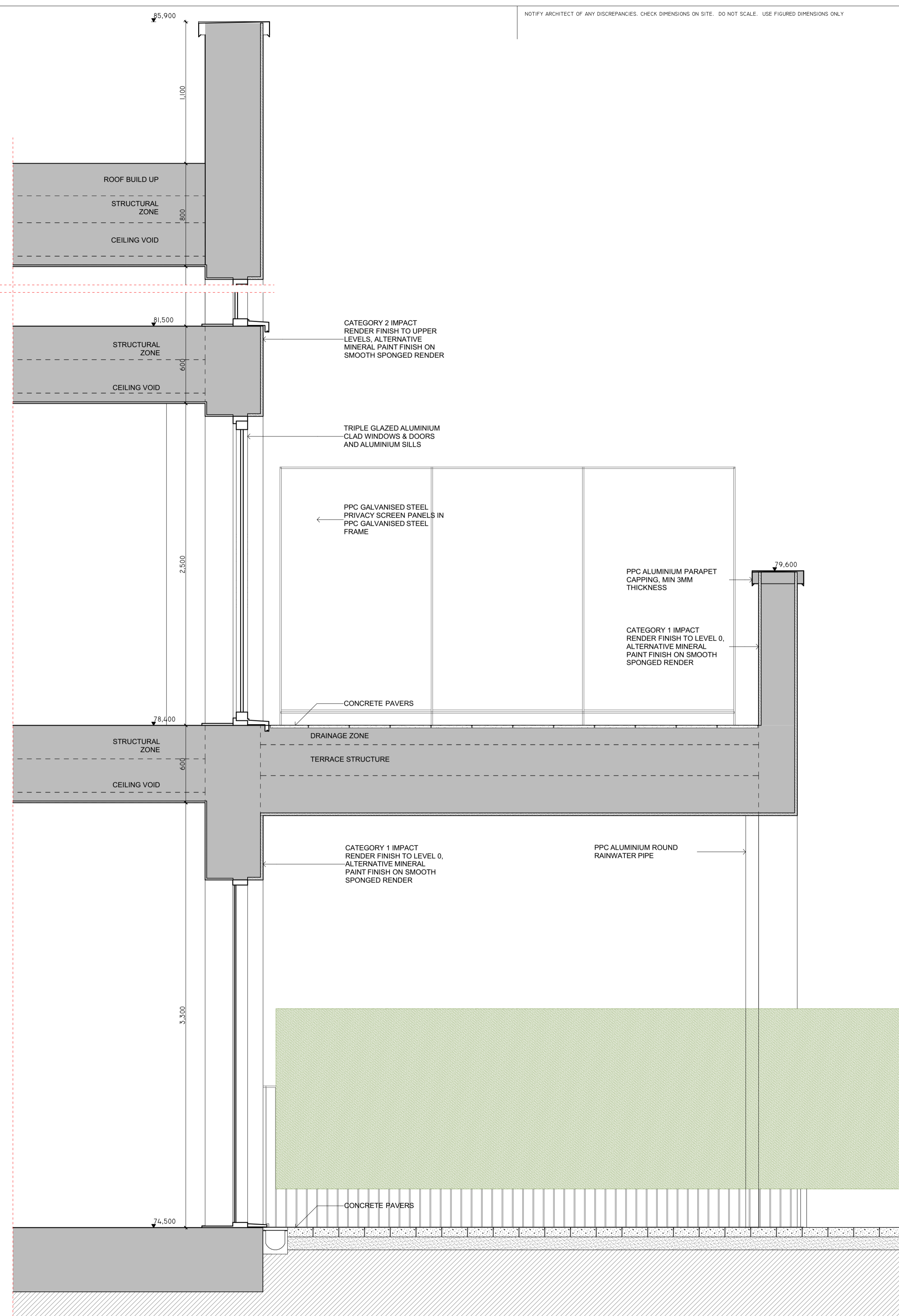
02 SECTION BLOCK C P4004 1:20
