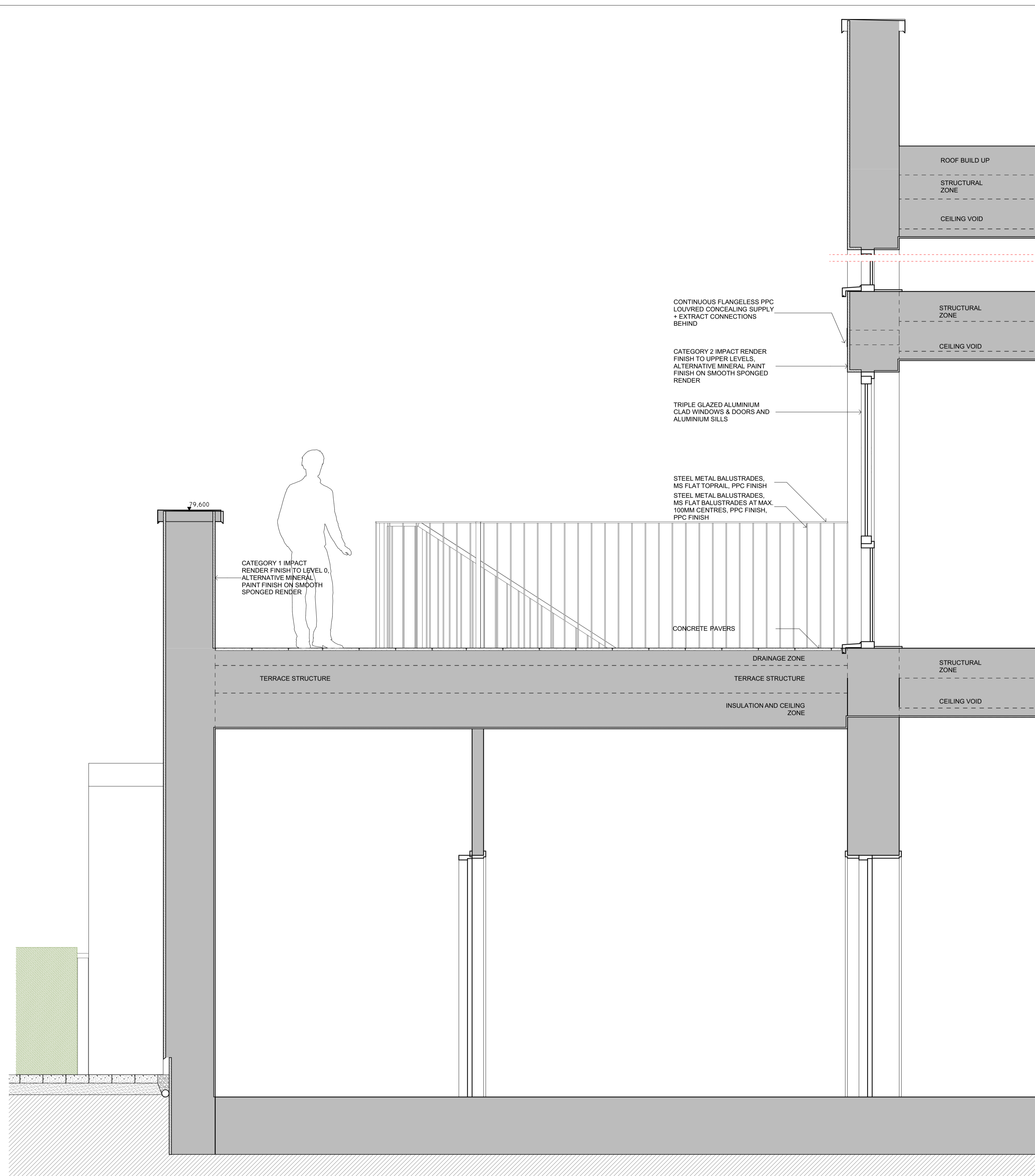
01 SECTION BLOCK C P4004 1:20
