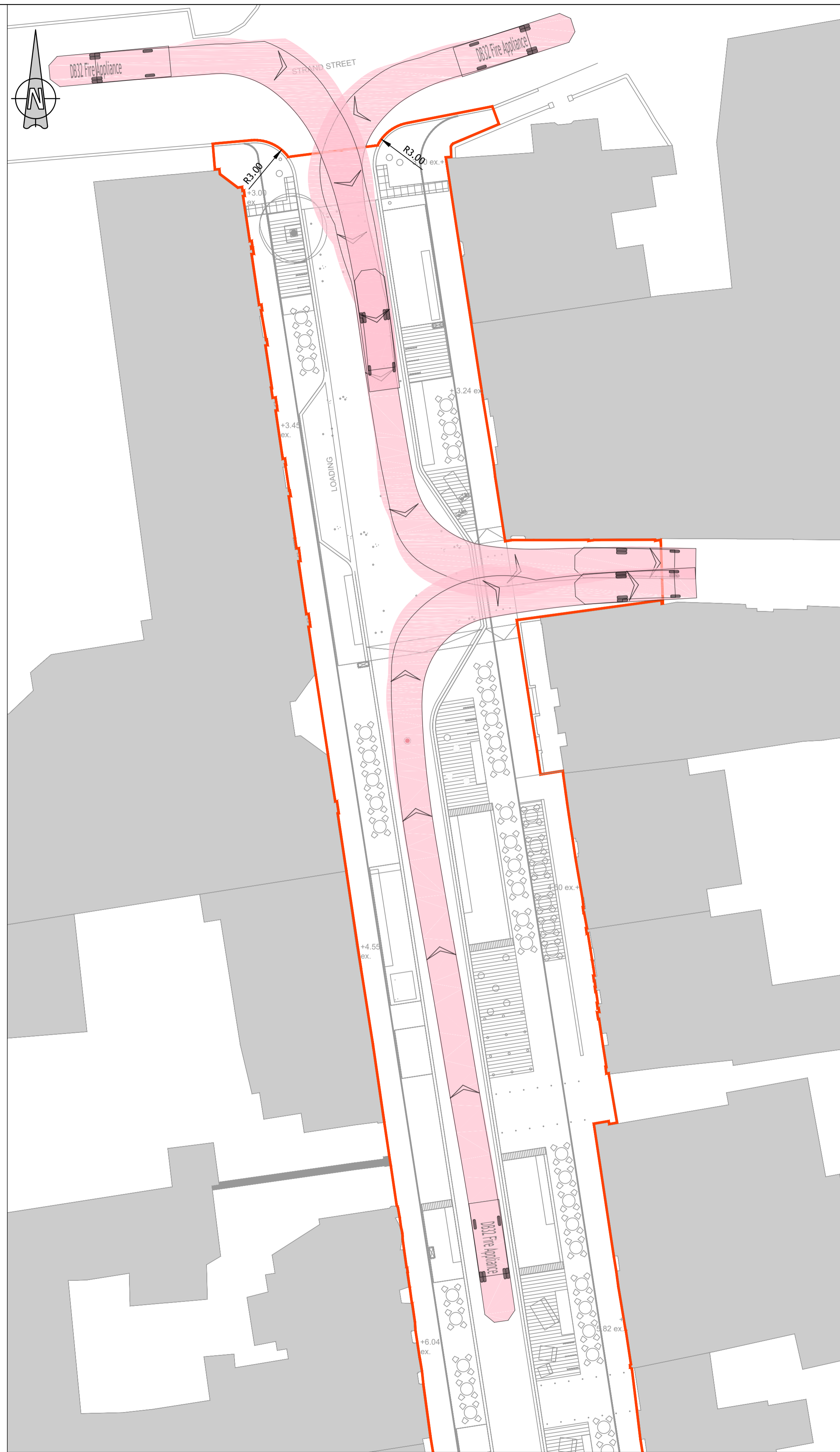
PLAN VIEW 3 SCALE 1:200
