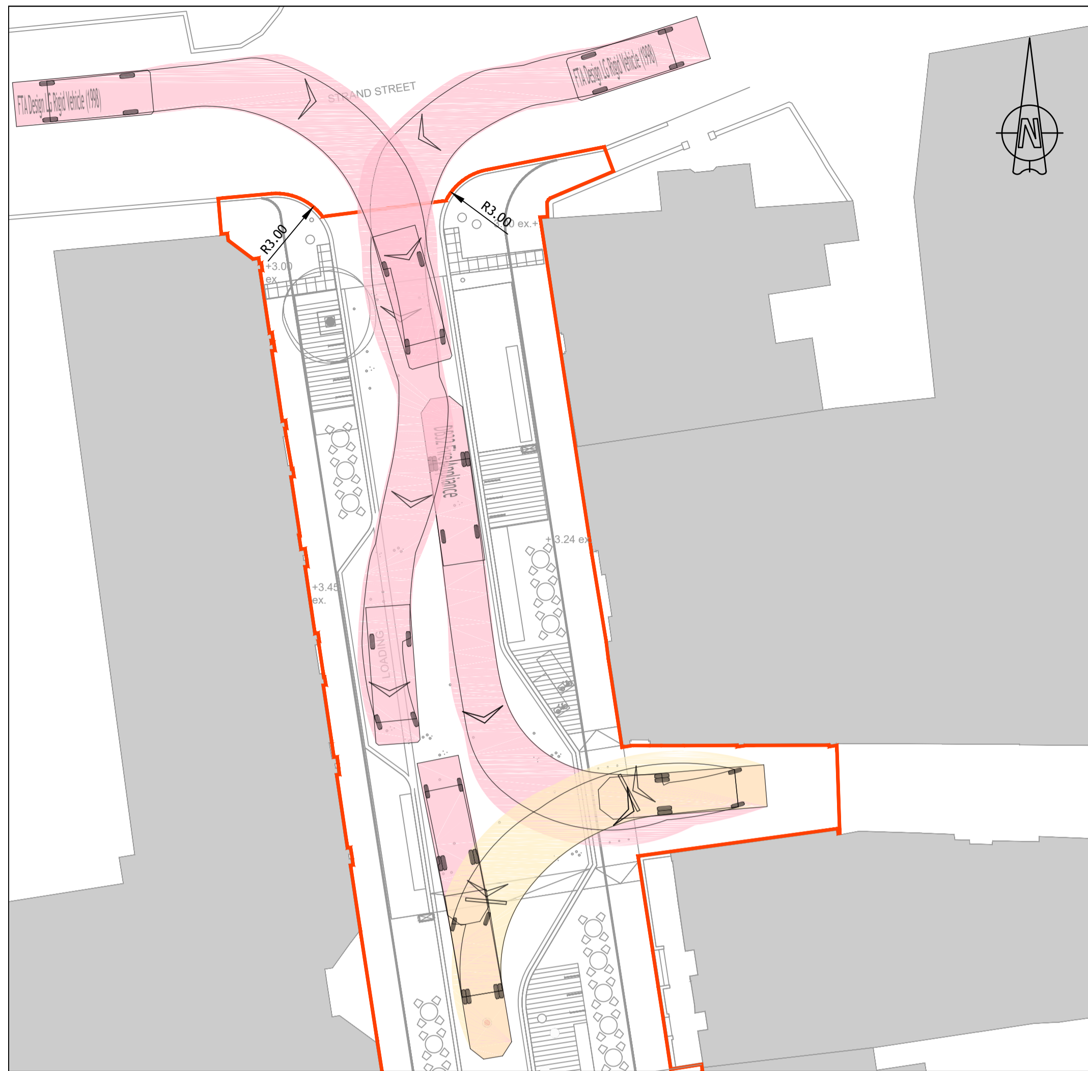
PLAN VIEW 1 SCALE 1:200
