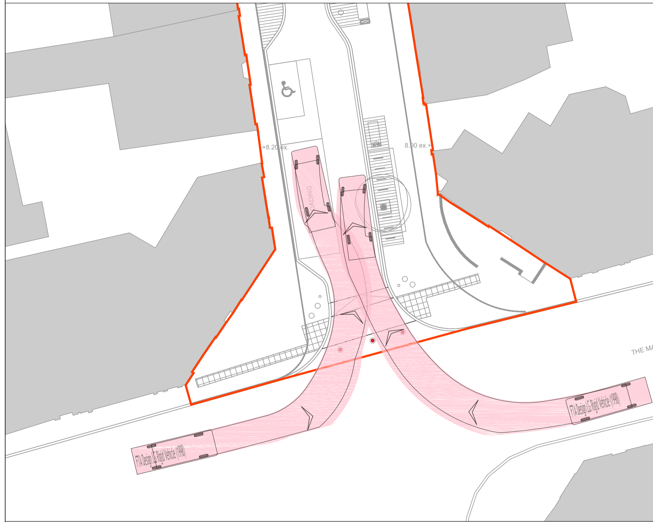
PLAN VIEW 2 SCALE 1:200
