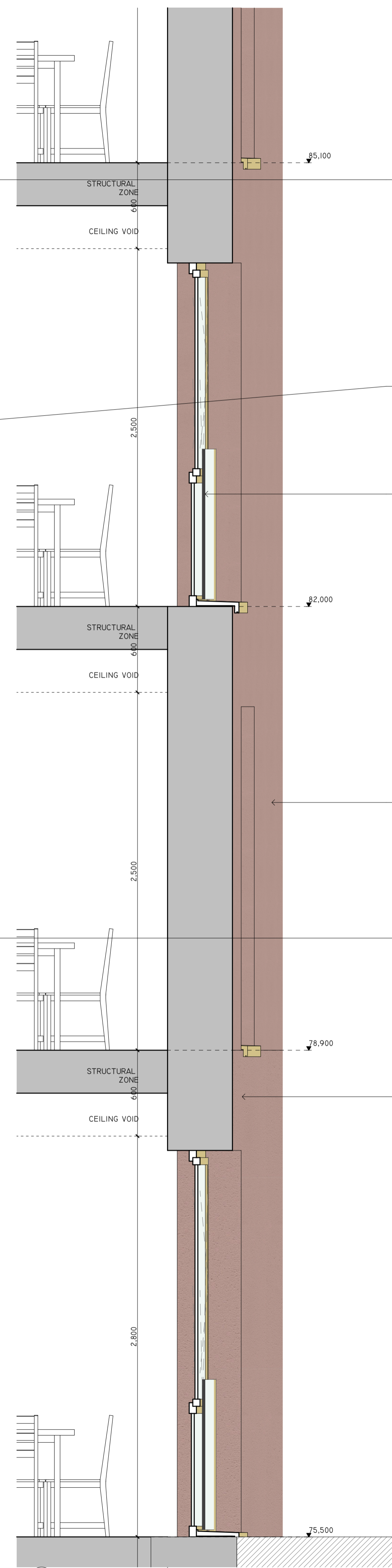
S-11 ACOUSTIC WINDOW SECTION 1:20
