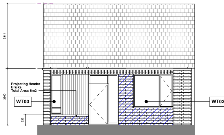
3 East Elevation_House Type A2 1 : 50
