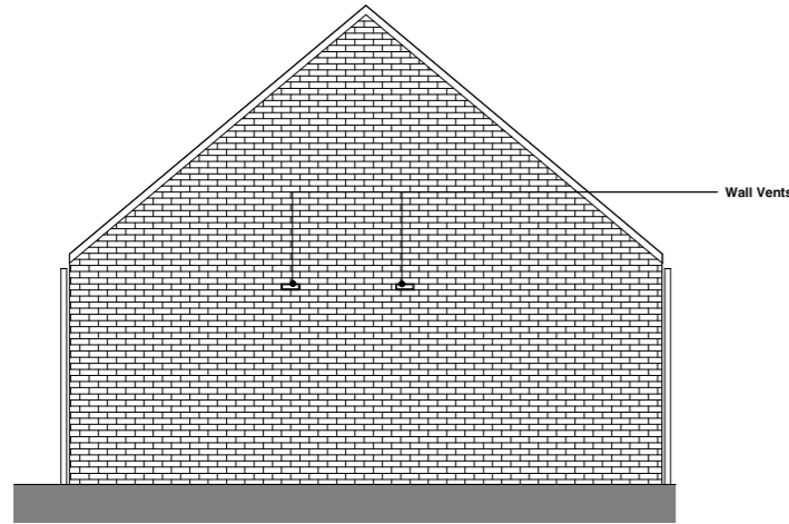
1 North Elevation_House Type A2 1 : 50
