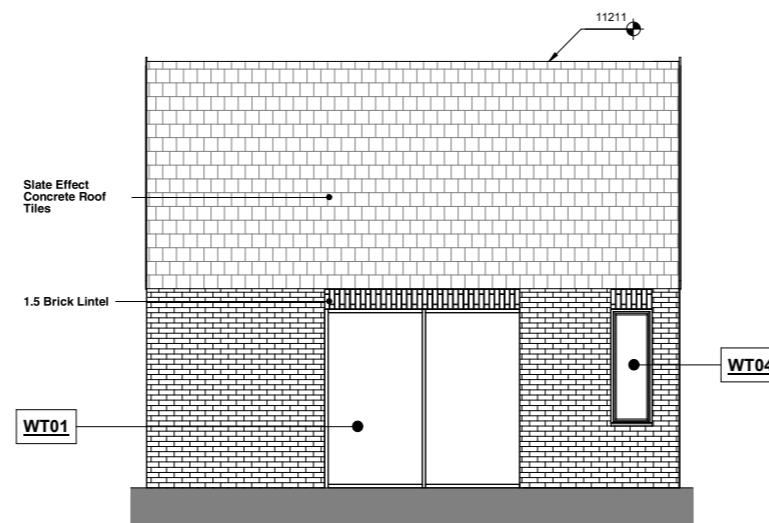
4 West Elevation_House Type A2 1 : 50
