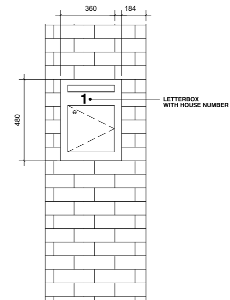
5 Elevation_Letterbox 1 : 10
