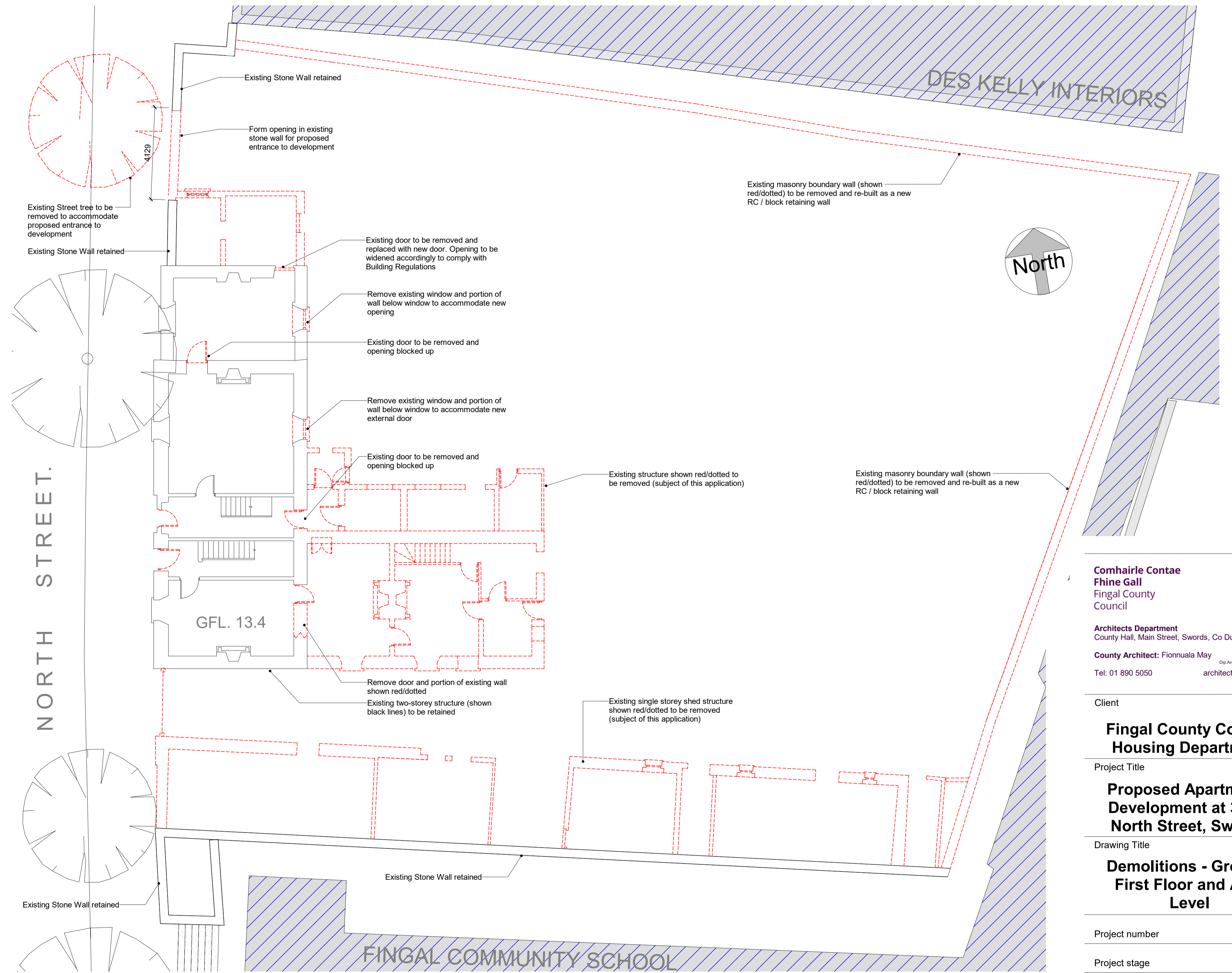
Demolition Ground Floor 1 : 100
