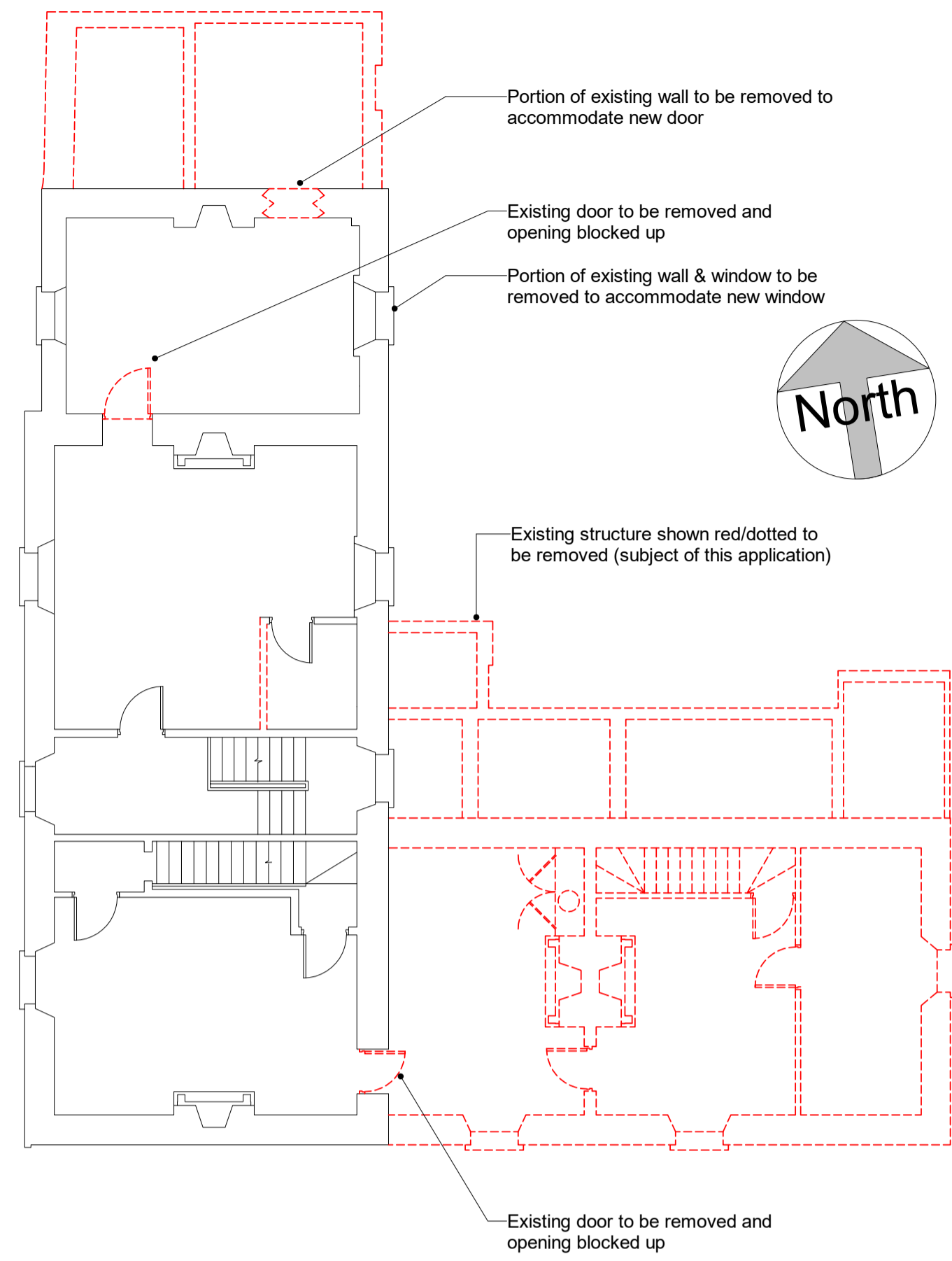
Demolition First Floor 1 : 100
