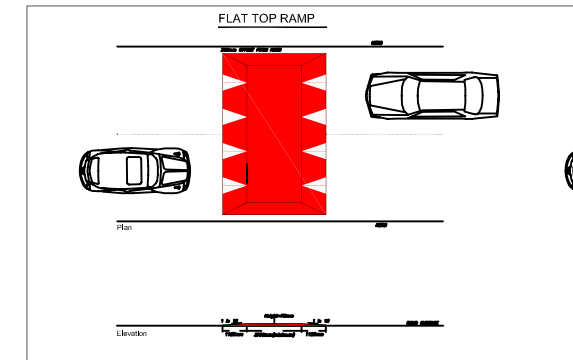
TYPICAL TRAFFIC CALMING BUS FRIENDLY RAMP DETAIL - 6m LONG
